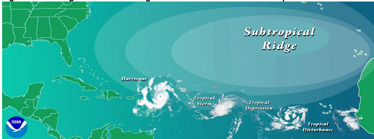
Figure 4.2.5-1 Progressive levels of organized disturbed weather in the tropics 113
