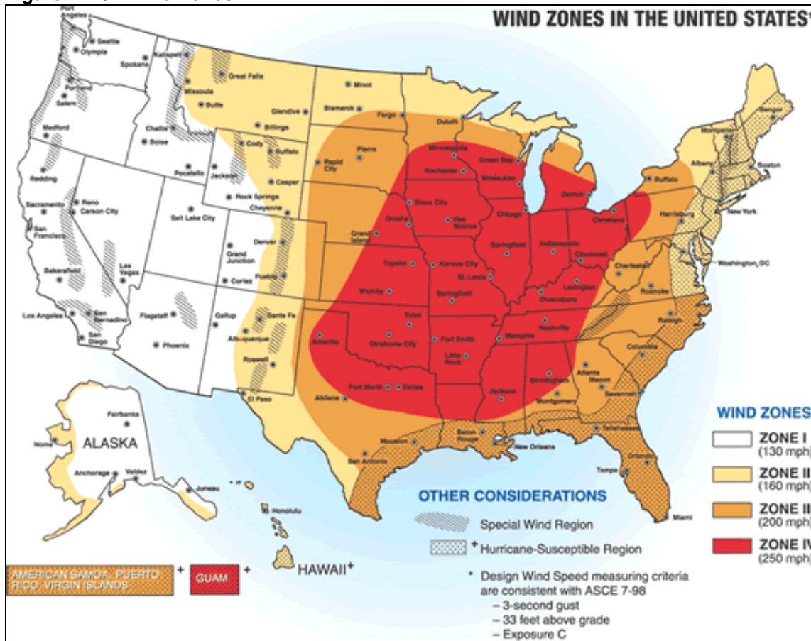
Figure 4.2.6-1 Wind Zones
