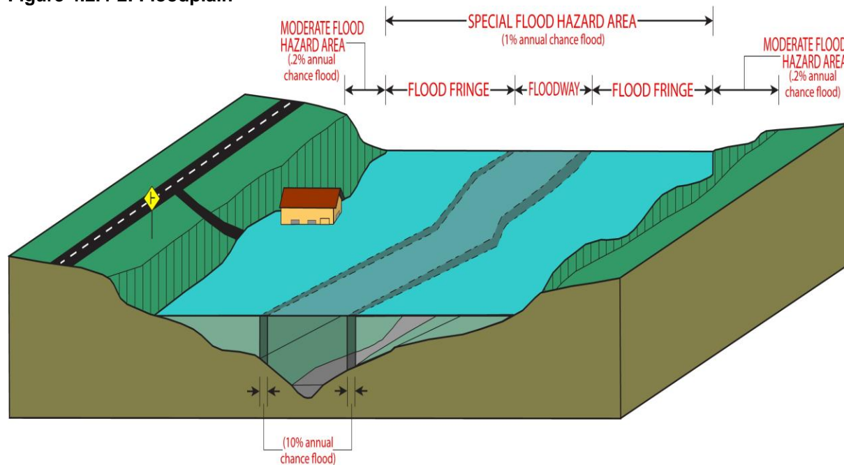
Figure 4.2.4-2: Floodplain
