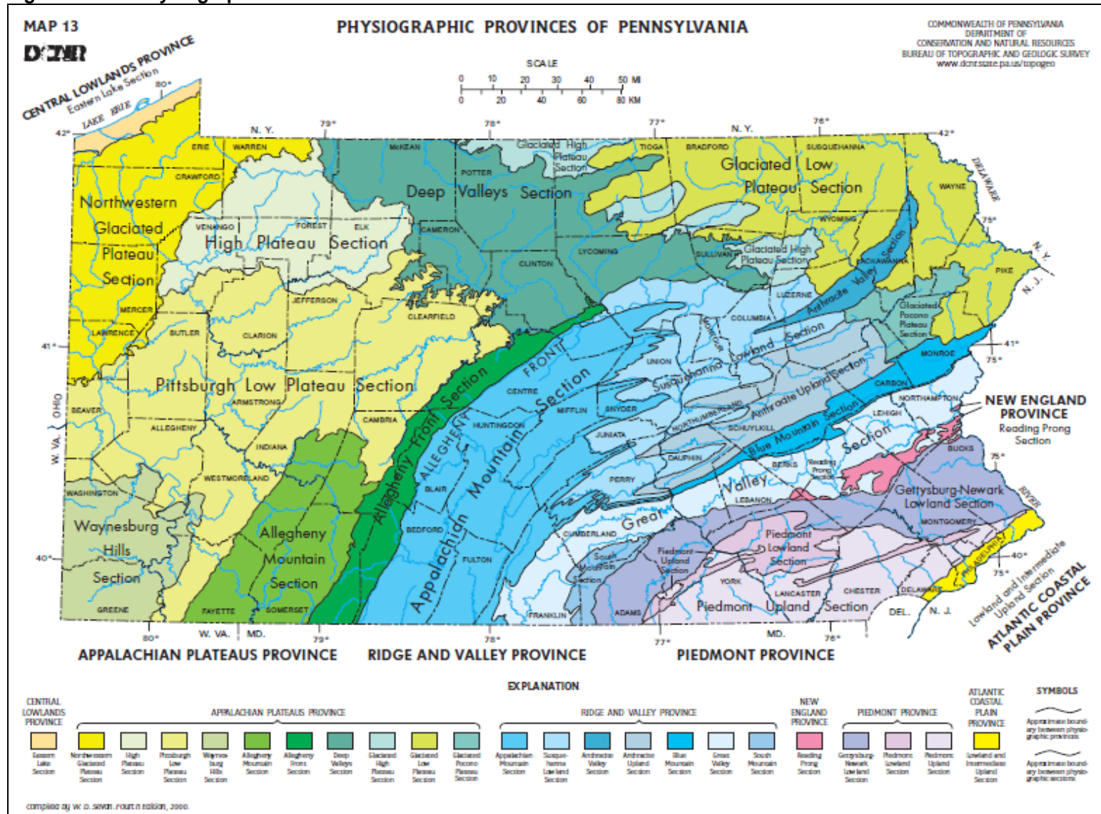
Figure 2.1.3-1 Physiographic Provinces
