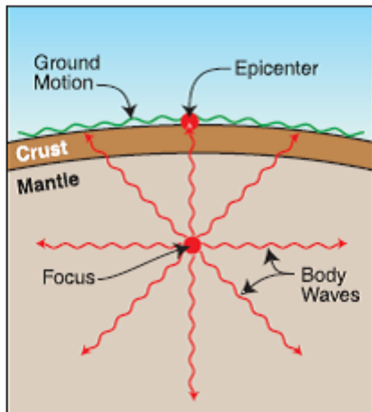
Figure 4.2.2-1: Earthquake Description
