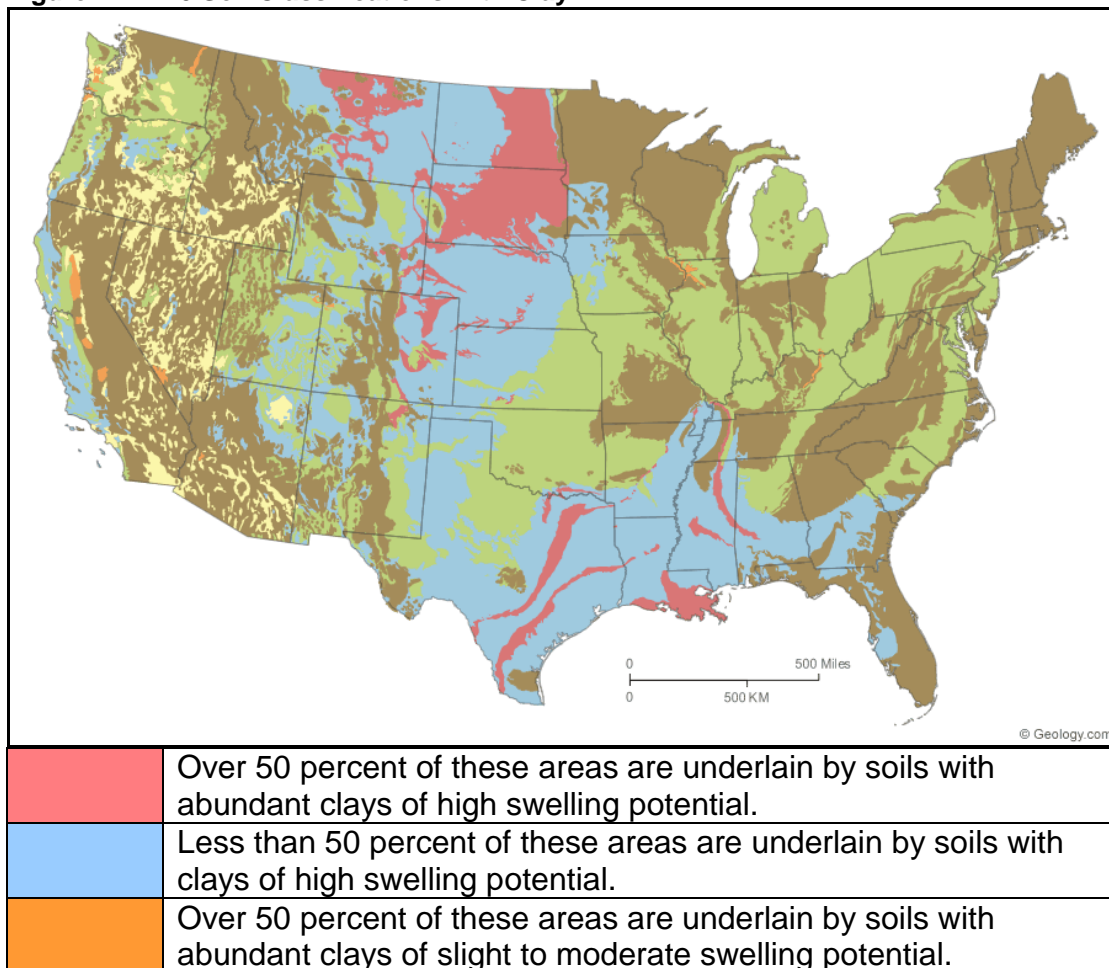
Figure 4.2.1-10 Soil Classifications with Clay
